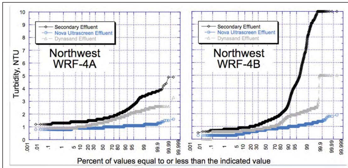
Figure 5.2 Comparison of the performance of two filters based on turbidity (Bourgeois et al., 2010).
