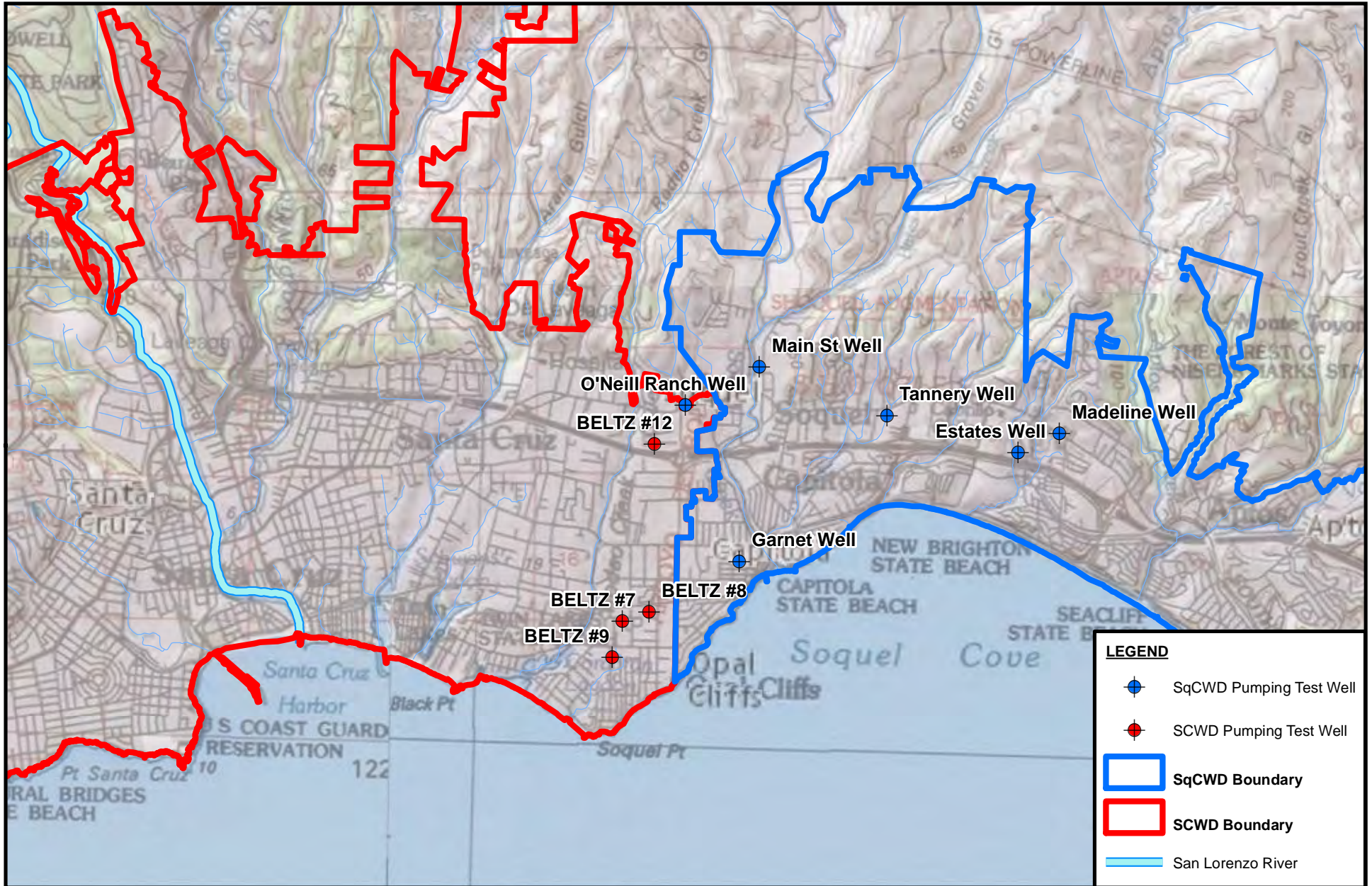
FIGURE 6. WELL LOCATION MAP - WESTERN PURISIMA AREA Reconnaissance-Level ASR Study Stratus Consulting / City of Santa Cruz WSAC
