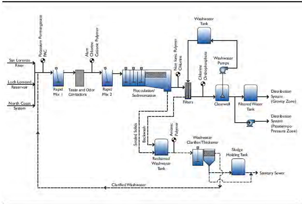
Figure 3-4. Process Flow Diagram of Graham Hill Water Treatment Plant
